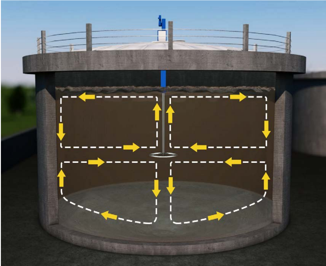
Figure 2: LM™ Mixer (showing flow pattern inside Digester) (Click Link to Watch Video)
